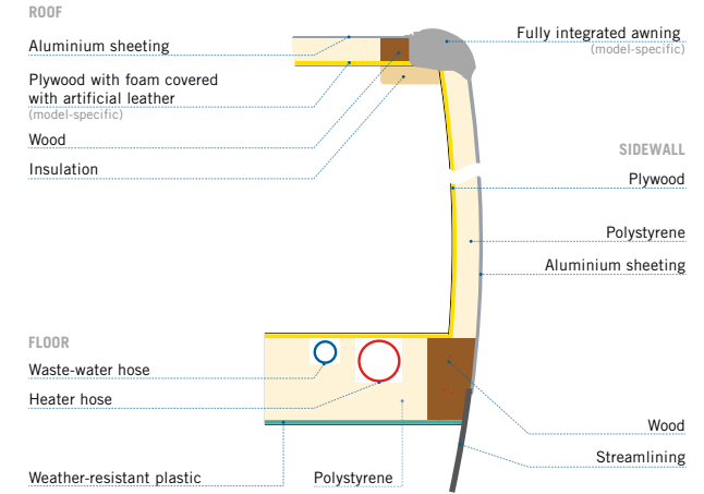
Cross-section: floor/sidewall of the Toskana/Toskana Exclusive range
